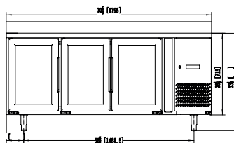
VISTA FRONTAL
