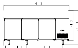
VISTA FRONTAL
